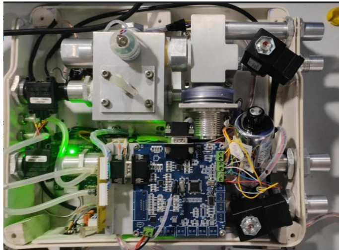
Assembled Ventilator Assist unit
